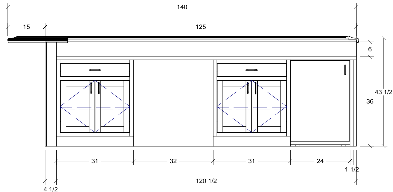
3 Elevation Back of Front Bar Scale: 1/2" = 1'
