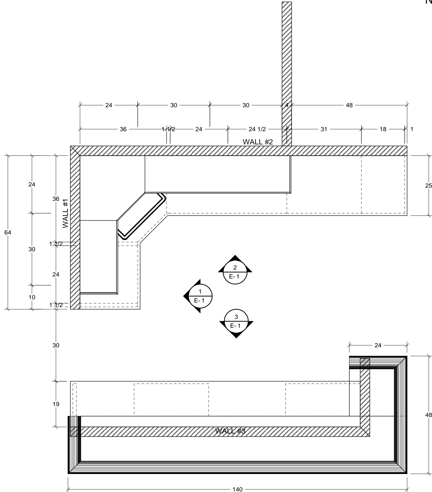
1 Plan View Scale: 1/2" = 1'
